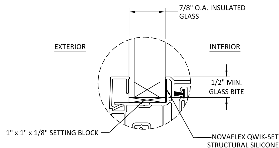
GLAZING DETAIL
