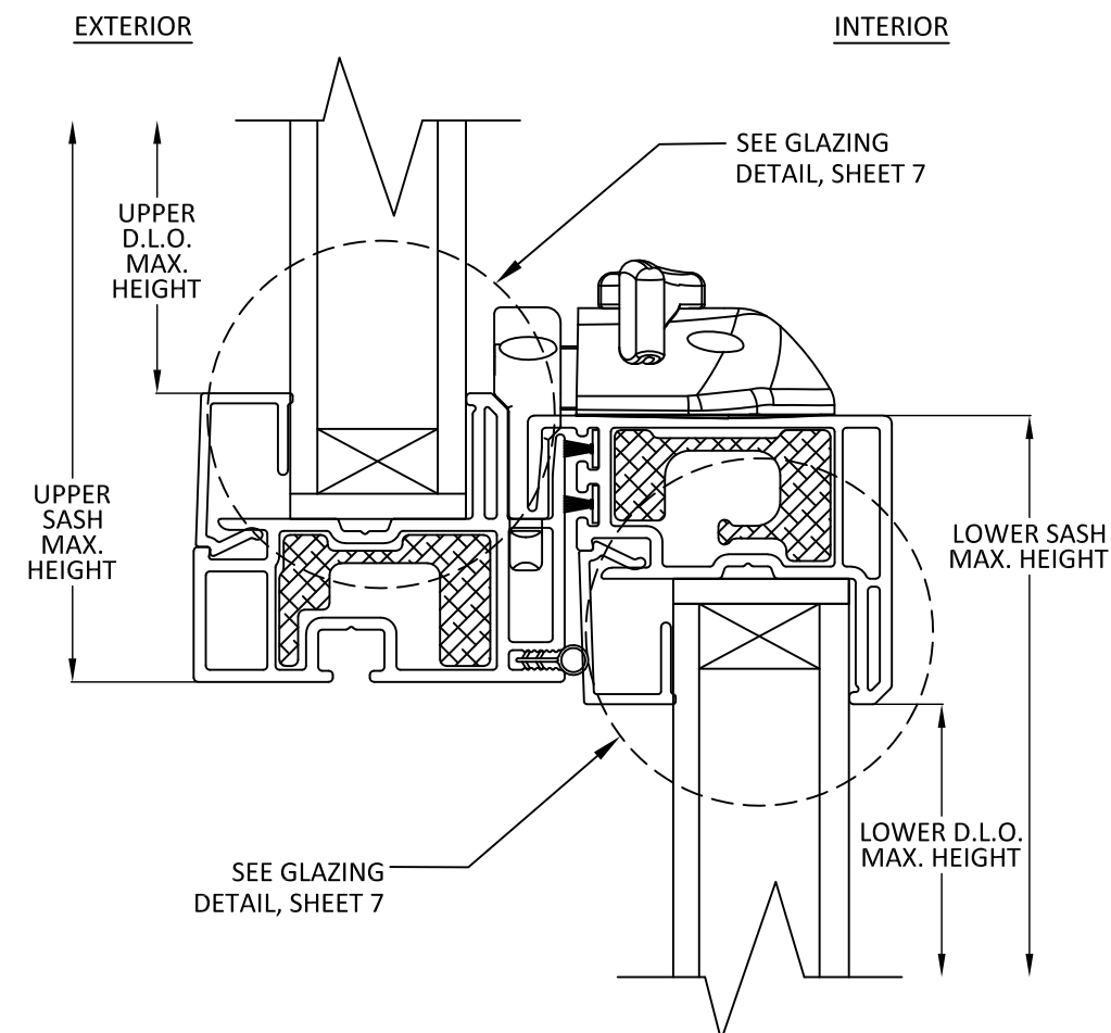
VERTICAL SECTION
