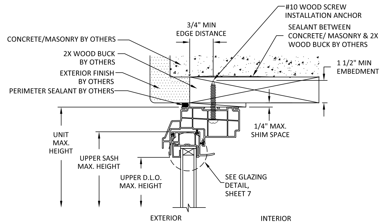
A 5 VERTICAL SECTION THROUGH FRAME INSTALLATION WOOD BUCK
